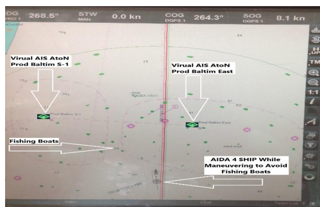
Figure (7): The ship Aida IV during the implementation of the practical experiment in the navigational passage Damietta - Burullus. Source: Photo by Transas ECDIS, Aida IV (1/2020)
